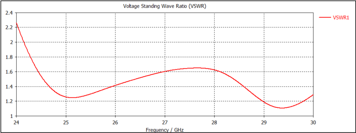
Figure 4. VSWR Measurements
