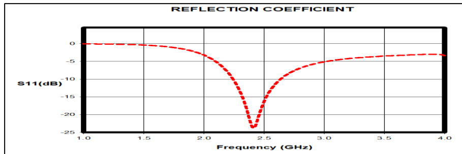
Figure 3. Reflection Coefficient
