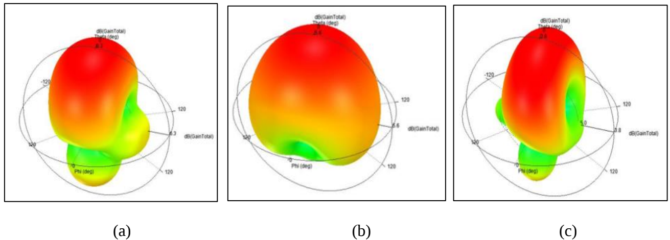
Figure 6. Gain Plot for Different Feed a) Proximity Coupled (b) Aperture Coupled (c) Inset Feed
