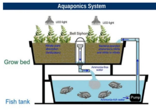
Figure 2. Aquaponic System [20]
