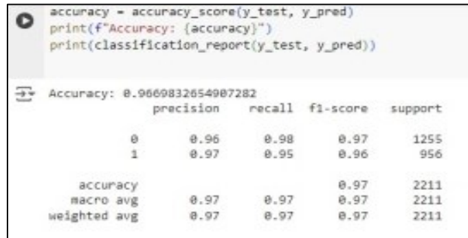
Figure 10. Performance of Random Forest
