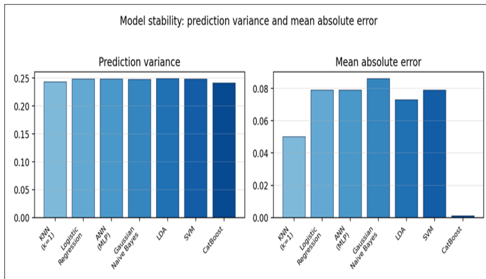
Figure 5. Prediction variance and mean absolute error across the seven candidate models
