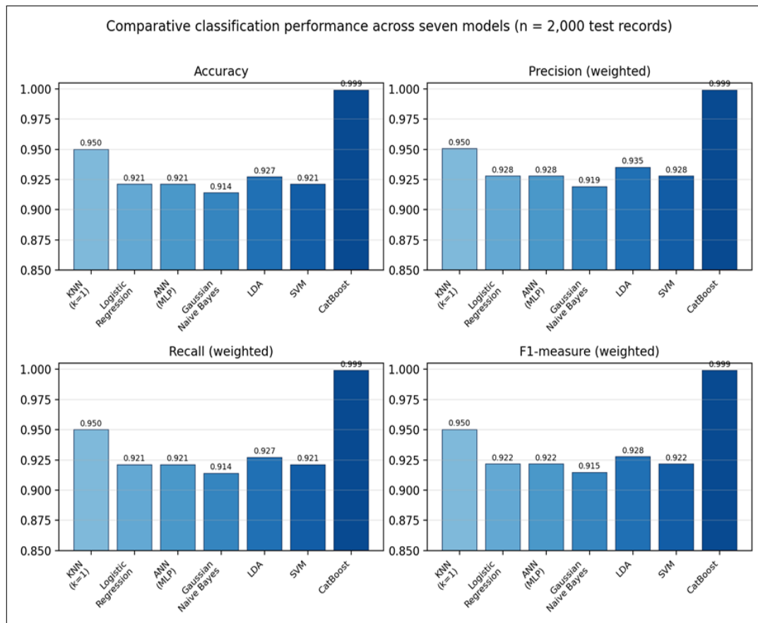
Figure 4. Comparative accuracy, precision, recall, and F1-score across the seven candidate models
