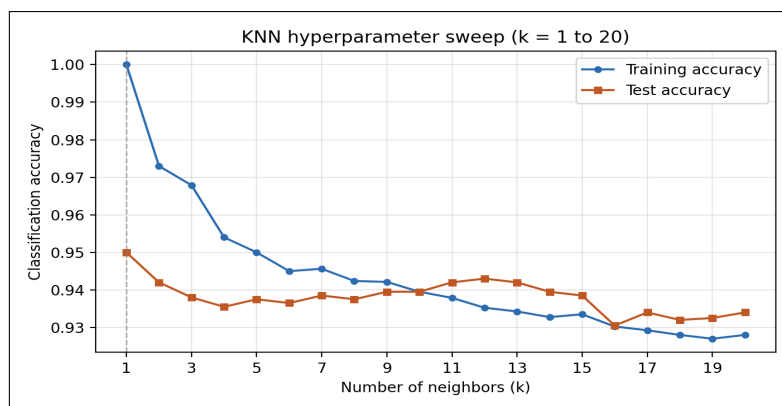
Figure 3. KNN training and test accuracy as a function of neighbor count k (real values, k = 1 –20)
