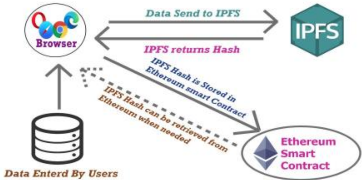
Figure 1. Workflow of DApp
