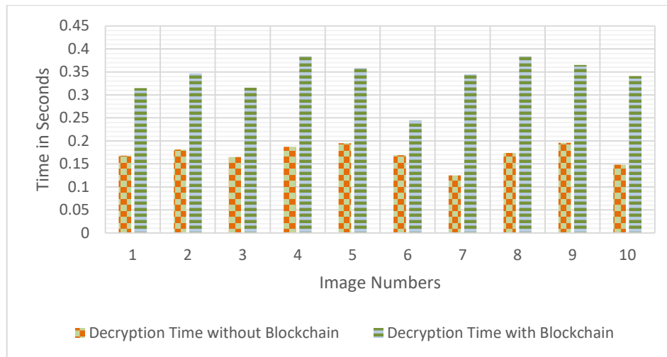
Figure 6. Comparison of decryption time with and without blockchain model
