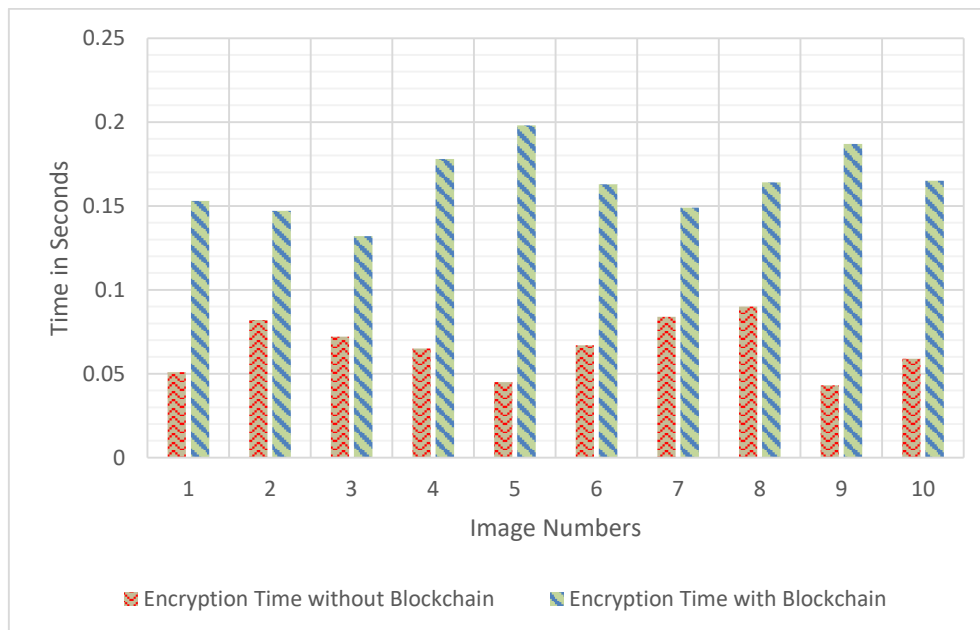
Figure 5. Comparison of encryption time with and without blockchain model
