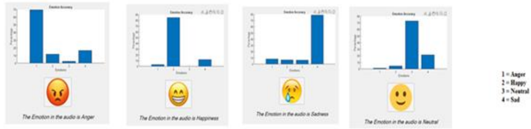
Figure 8. SVM Classifier
