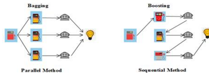
Figure 4. Ensembling Technique
