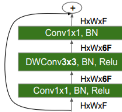
Figure 9. MBConv6, 3x3 [9]
