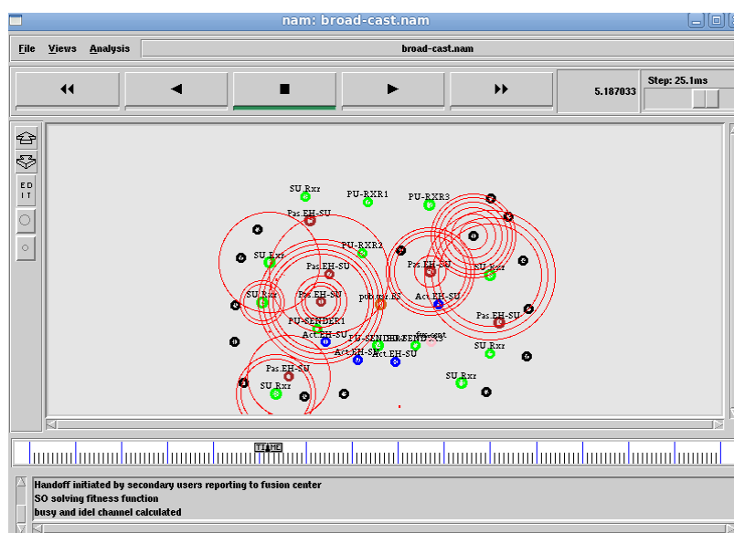
Figure 4.4. Fitness Evaluation
