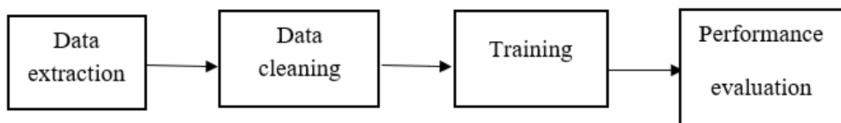
Figure 5. Linear Regression Procedure
