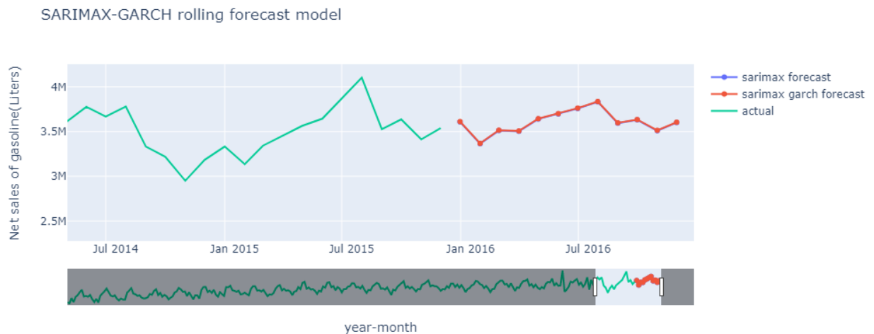
Figure 6: Forecast for Next 12 Month
