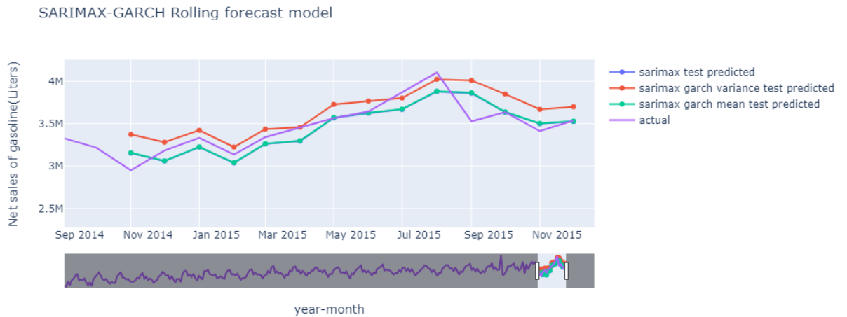
Figure 5. Prediction on Test Part using MODEL((1,1,0),(1, 0, 1, 12), "GARCH", 1, 1, 2, 'normal')
