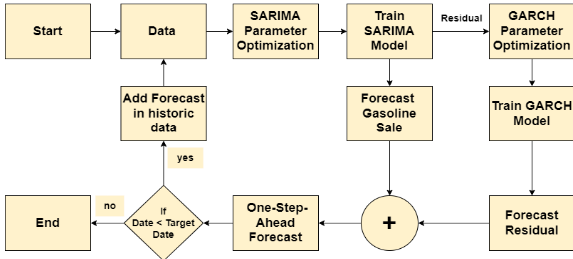
Figure 3. Flowchart of the Procedure for Hybridization of SARIMA and GARCH Model.
