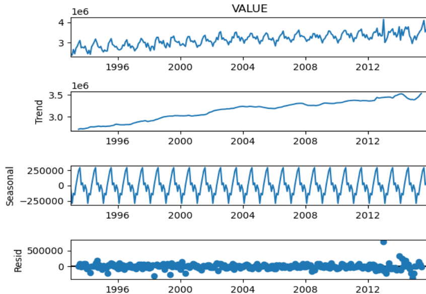
Figure 2. Sale of Gasoline in Canada (1993-2015) Time Series Decomposition
