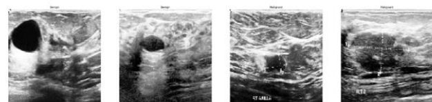
Figure 6. Histogram Equalization
