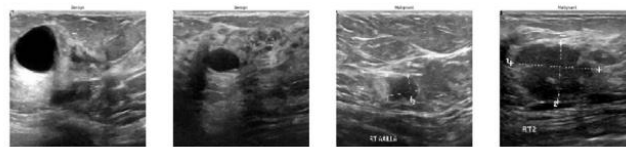
Figure 5. Grayscale Conversion
