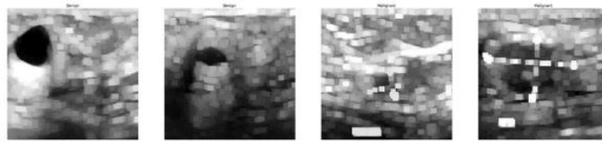
Figure 11. Dilation
