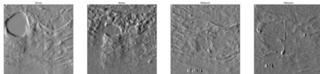
Figure 9. Sobel Filter
