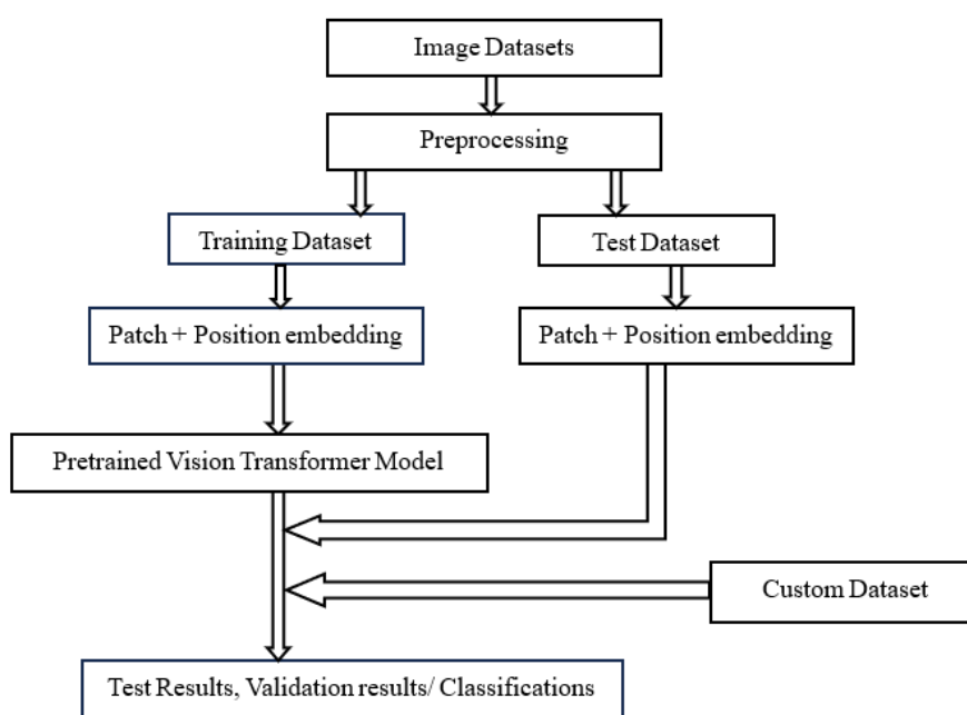
Figure 1. Workflow for Potato Leaf Disease Classification
