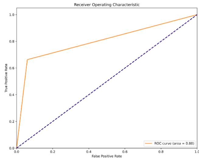
Figure 6. ROC Curve of MLP Model
