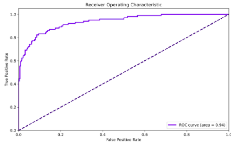
Figure 7. ROC Curve of LSTM Model
