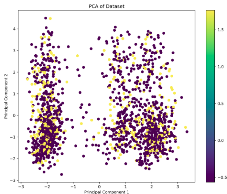
Figure 3. PCA – Feature Scaling Analysis
