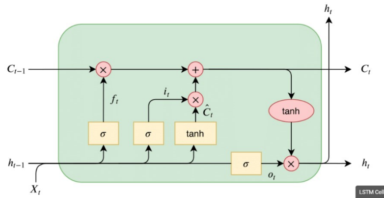
Figure 5. LSTM Model Architecture [10]
