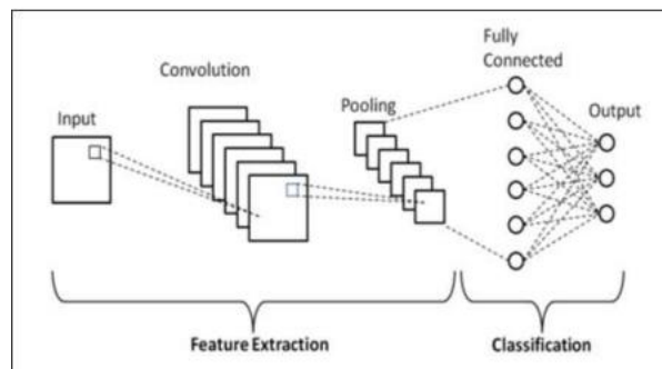
Figure 4. CNN Architecture
