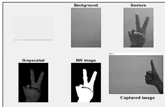
Figure 2. Image Pre-Processing
