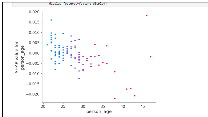
Figure 13. SHAP Outputs
