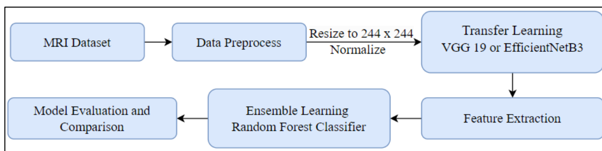
Figure 2. Flow of Proposed Approach
