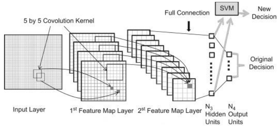
Figure 3 Hybrid Framework of our proposed system
