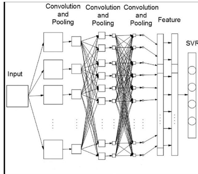
Figure 4 Internal Convolution and pooling structure of framework
