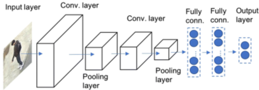
Figure 6 Experimental Setup of Classification Procedure
