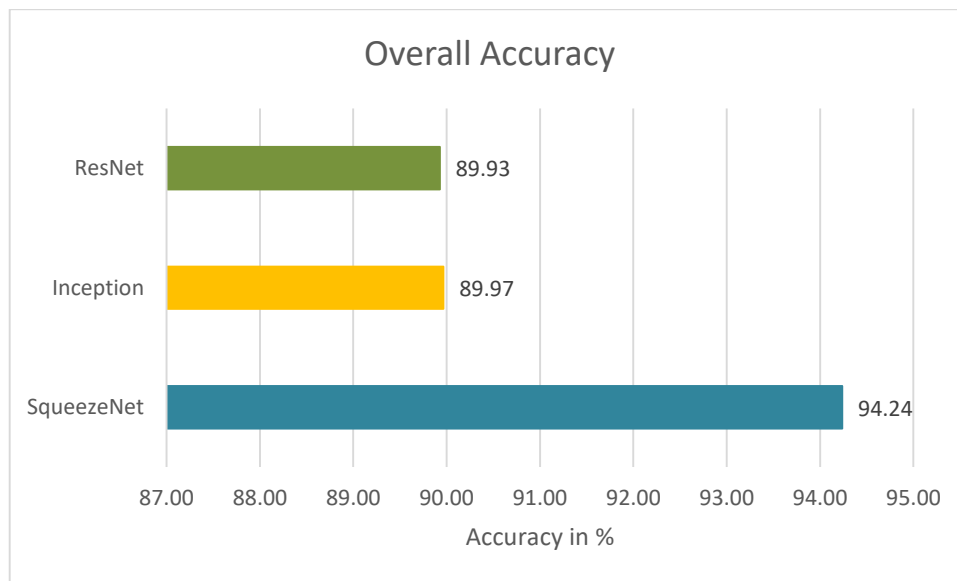
Figure 8. Overall accuracy comparison among the verified algorithms
