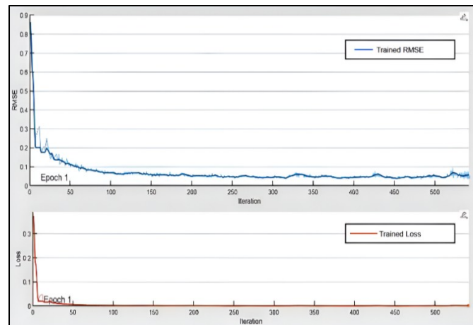
Figure 3. RMSE Graph
