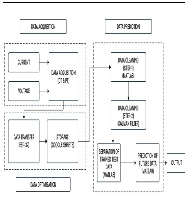
Figure 1. Proposed Block Diagram for Energy Optimization
