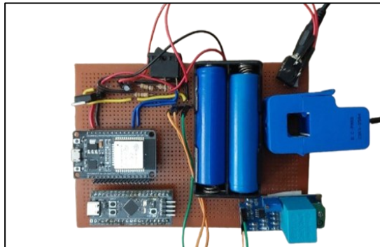
Figure 4. Hardware Prototype
