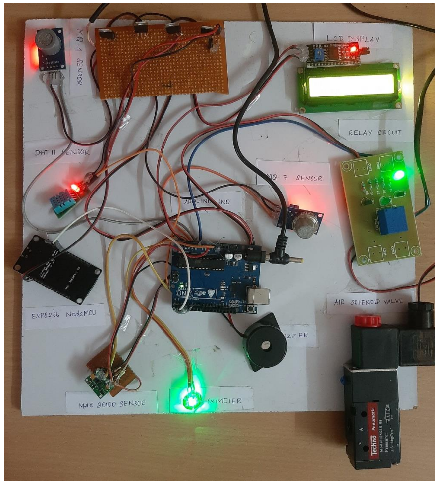
Figure 2. Hardware Setup
