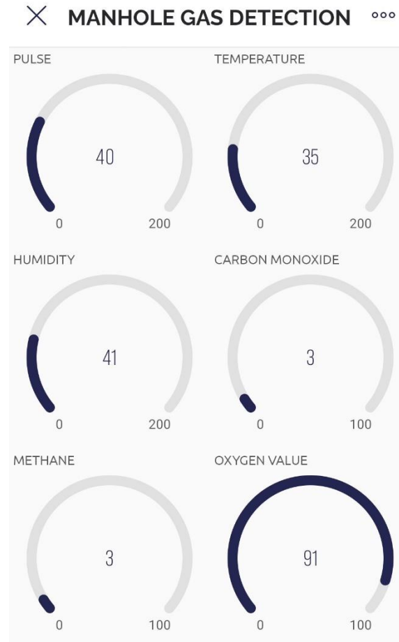
Fig 9. All sensor's data displayed in Blynk Application
