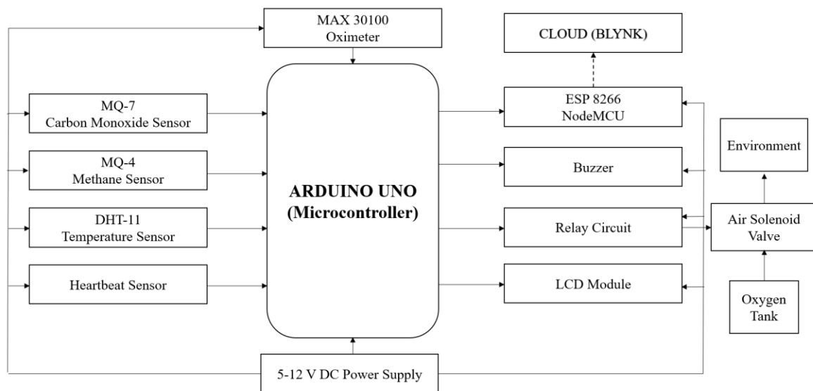
Figure 1. Block Diagram
