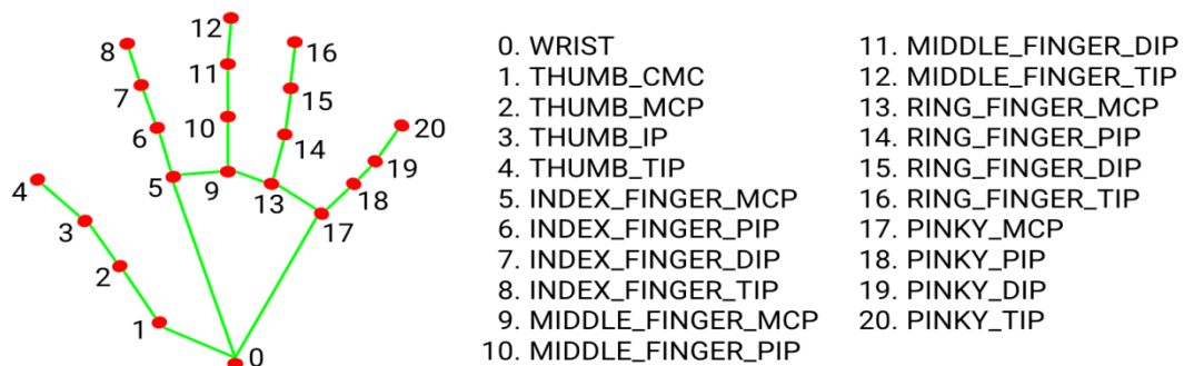
Figure 3. Hand Landmarks.
