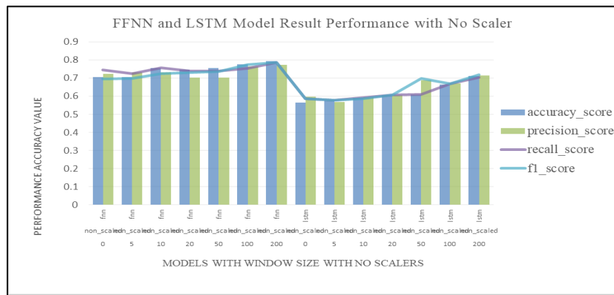
Figure 7. FFNN and LSTM Performance with No Scaler
