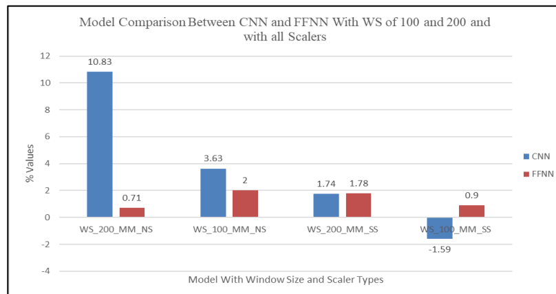
Figure 6. CNN and FFNN model with all Scalers
