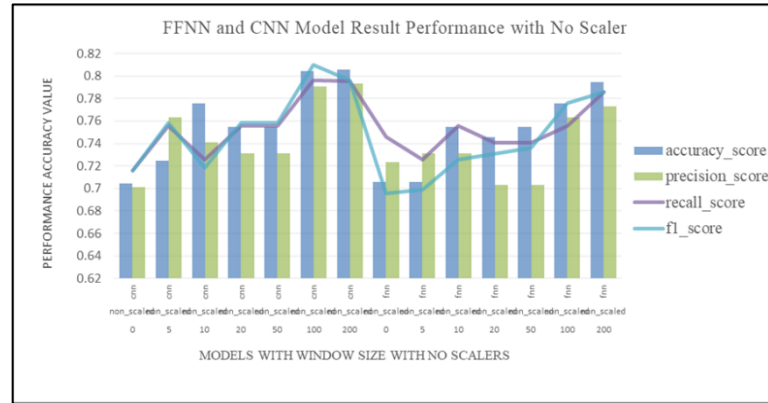
Figure 5. FFNN and CNN Performance with No Scaler
