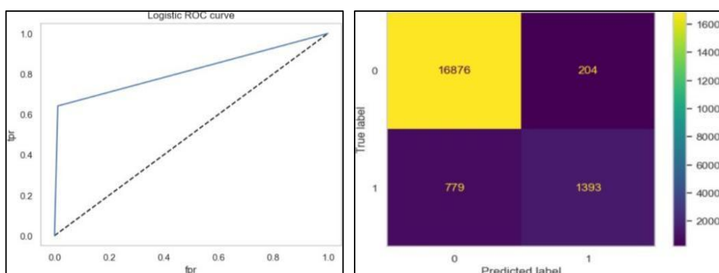
Figure 3. ROC Curve of Logistic Regression Tree and Confusion Matrix
