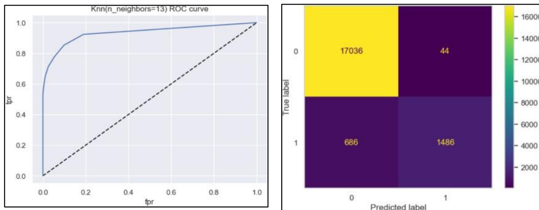
Figure 7. ROC Curve of KNN and Confusion Matrix
