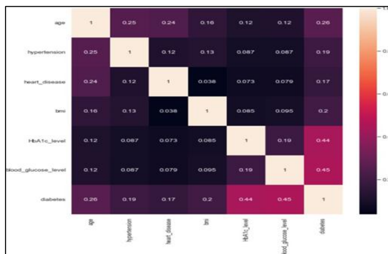
Figure 8. Correlation Matrix
