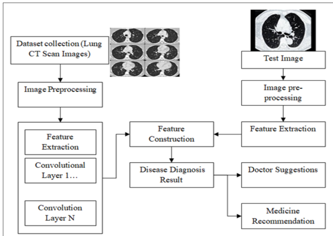
Figure 1. Overall methodology flow of the proposed lung CT image classification system.
