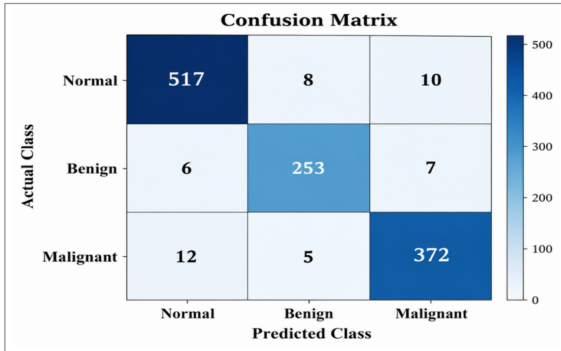
Figure 2. Confusion matrix for lung CT image classification.
