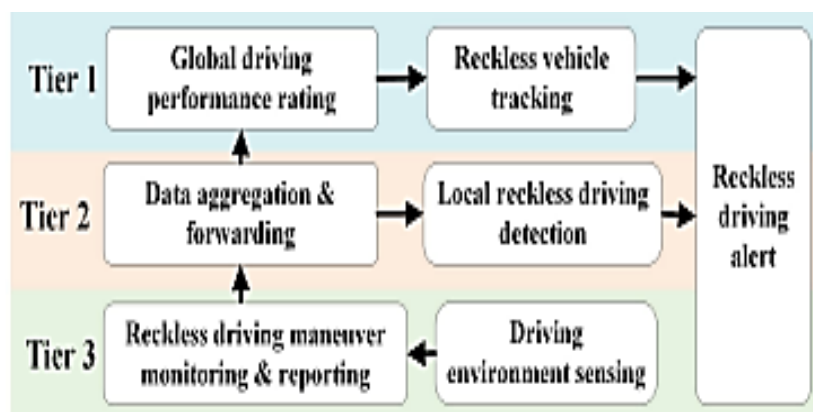
Figure 2. Three-layer System for Vehicle Speed Monitoring [3]
