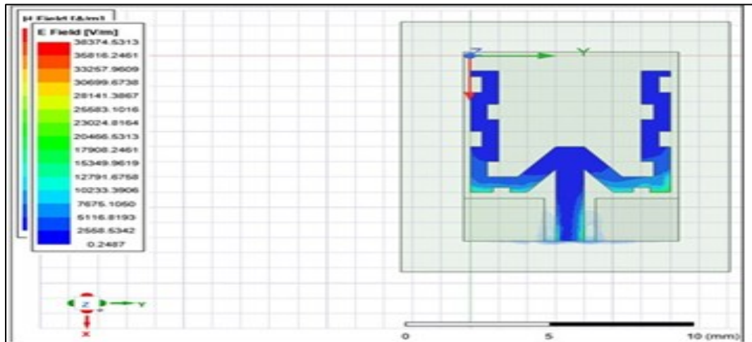
Figure 9. Field Distribution Pattern
