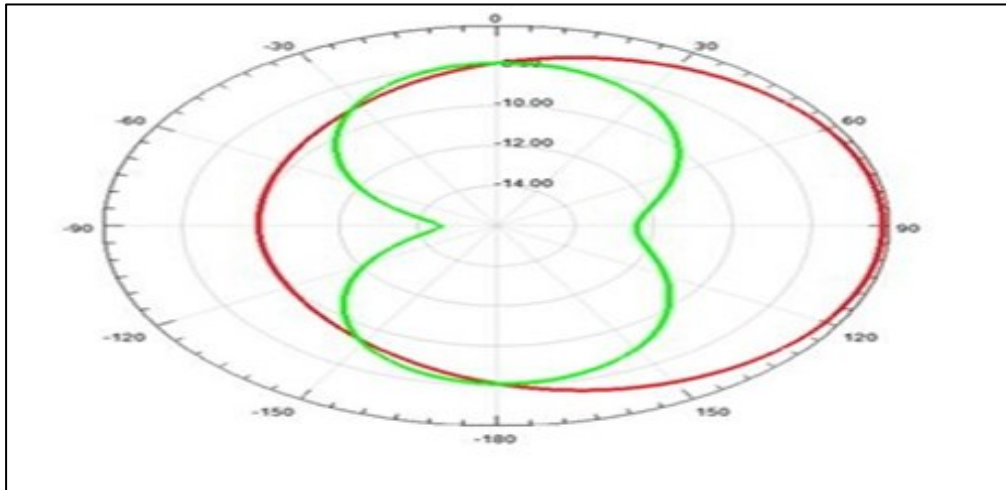
Figure 7. 2D Gain Plot
