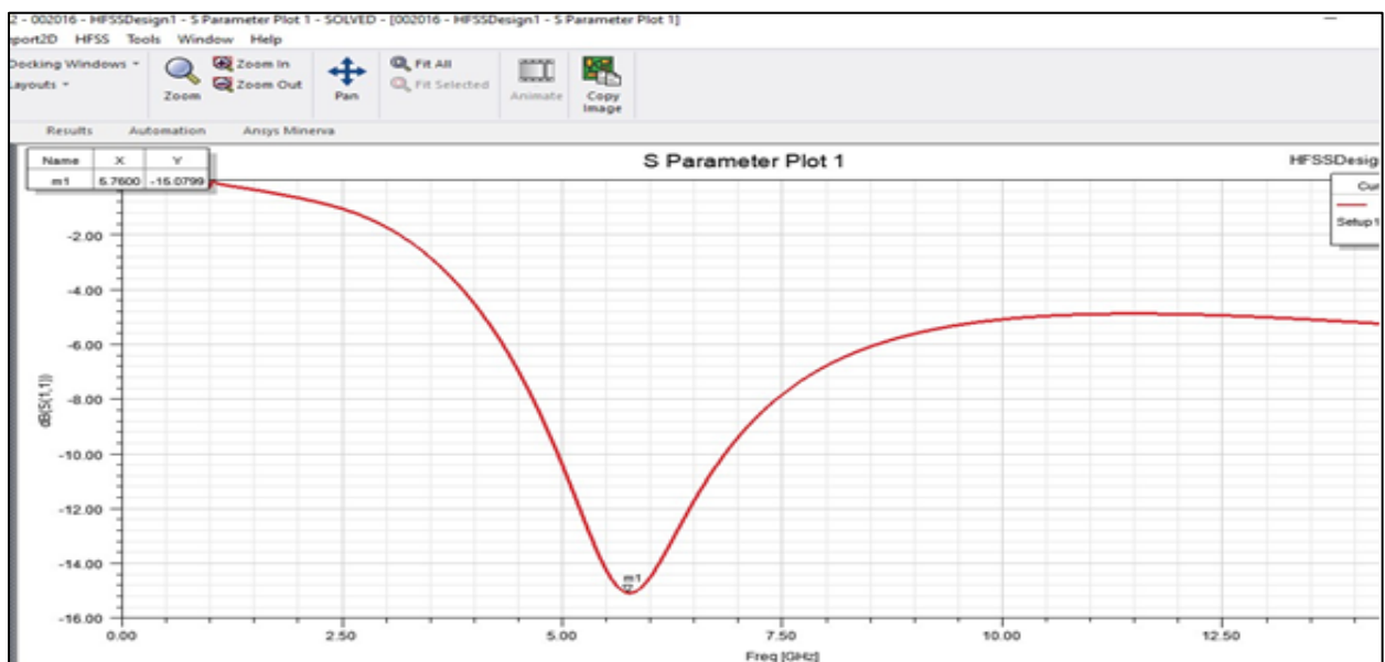
Figure 5. S-Parameter
