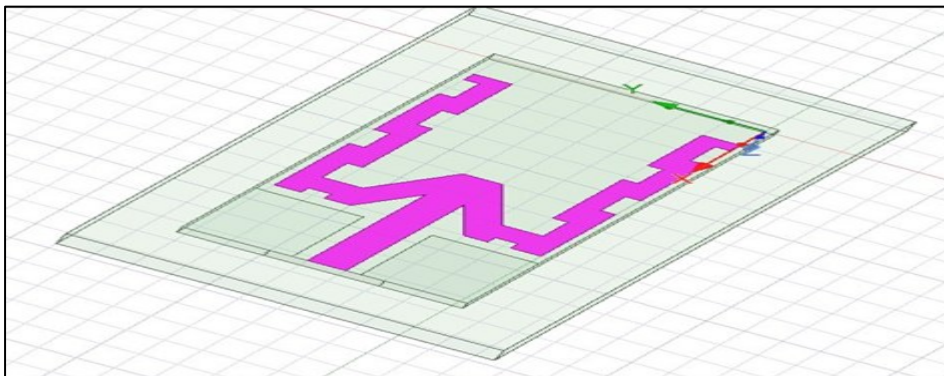
Figure 1. W-Shaped Meander Line Antenna
