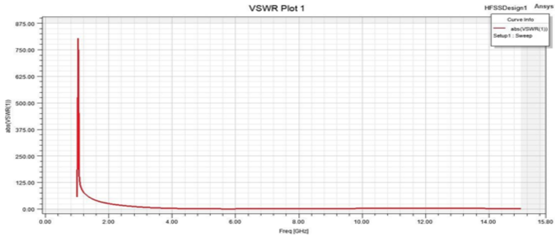
Figure 6. VSWR Plot
