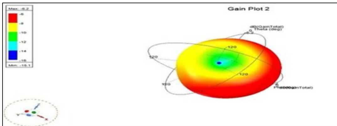
Figure 8. 3D Gain Plot
