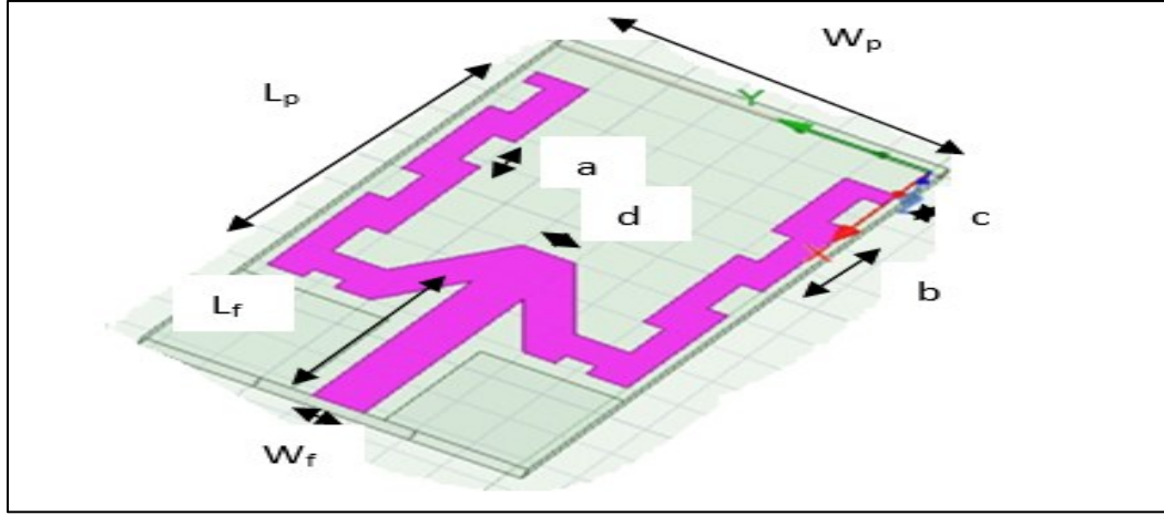
Figure 2. ZIG ZAG Pattern Structure of Antenna
