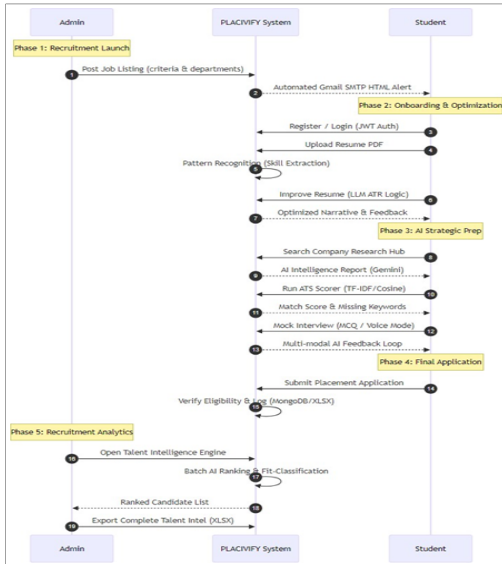
Figure 7. End-to-end PLACIVIFY process flow (student and admin swimlanes)
