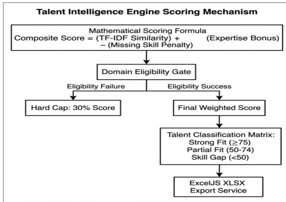
Figure 5. Talent intelligence engine scoring and classification
