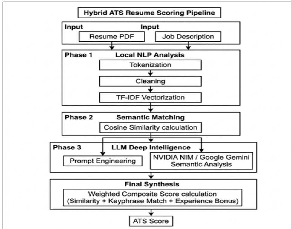
Figure 3. Hybrid ATS resume scoring pipeline
