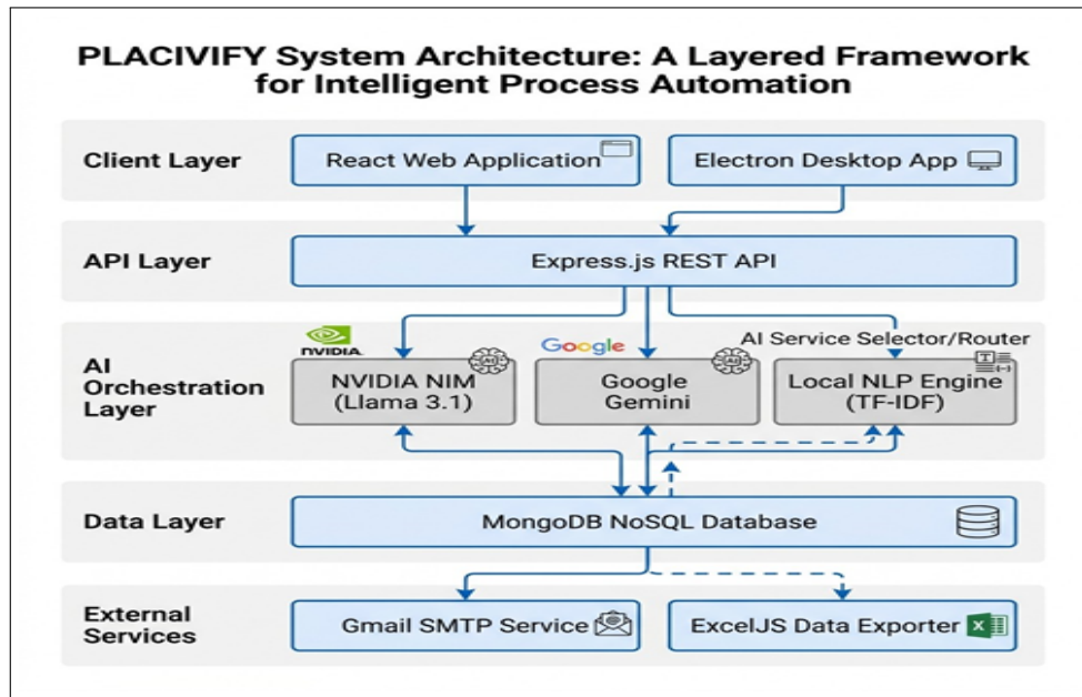
Figure 1. PLACIVIFY system architecture
