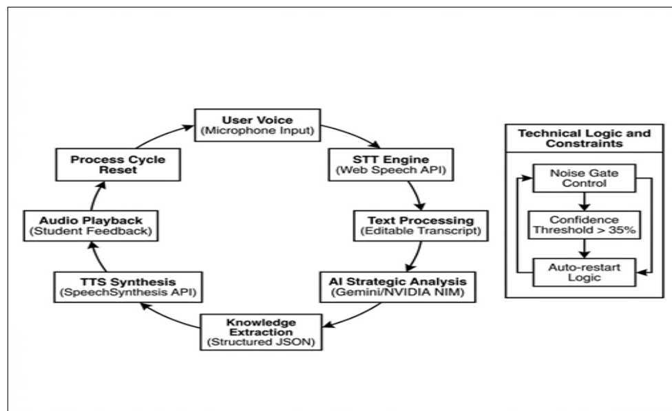
Figure 4. Voice mock interview speech-to-speech loop
