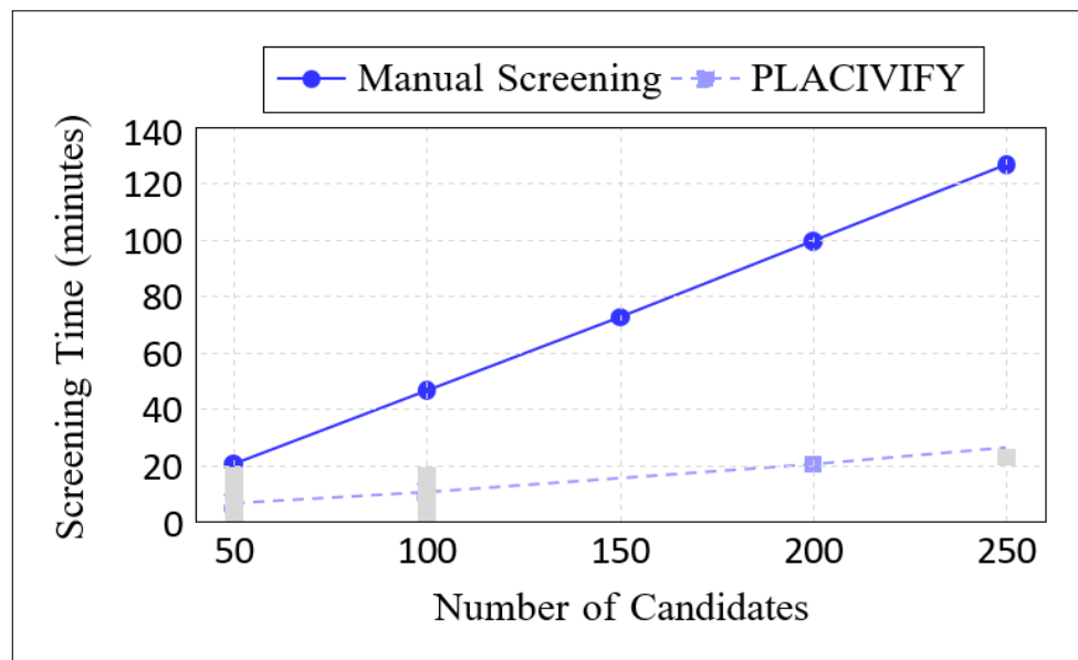
Figure 8. Scalability analysis of candidate screening
