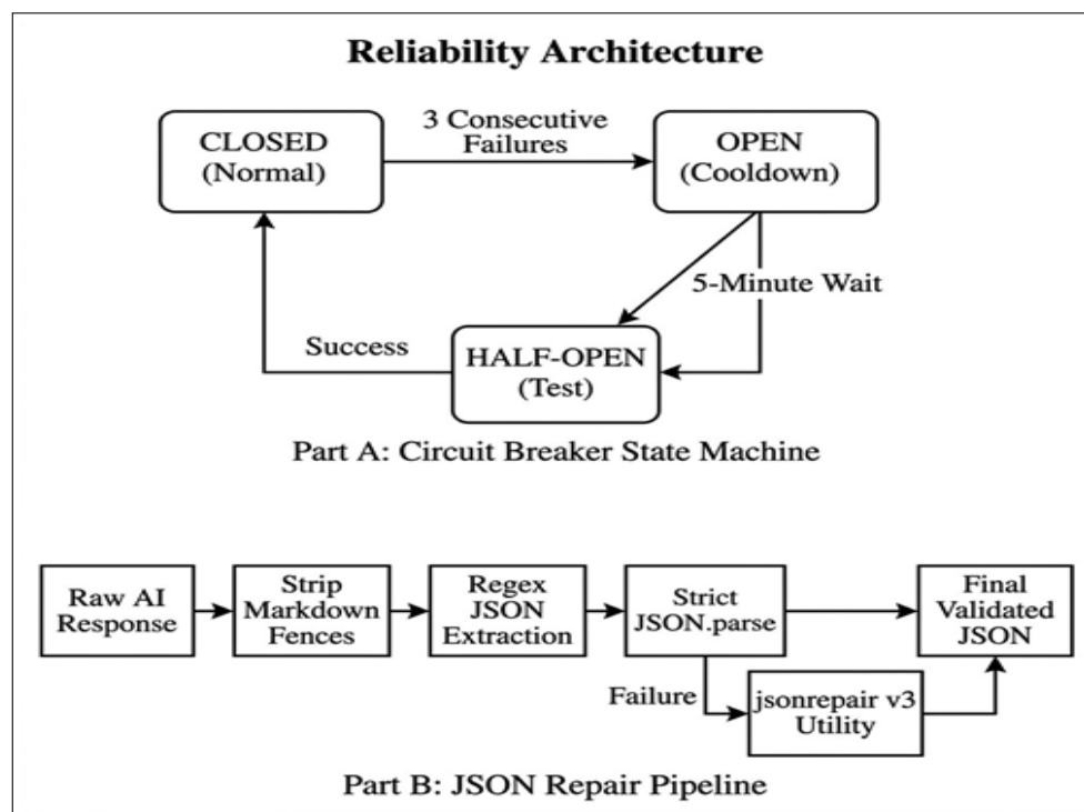
Figure 6. Circuit breaker state machine and JSON repair pipeline
