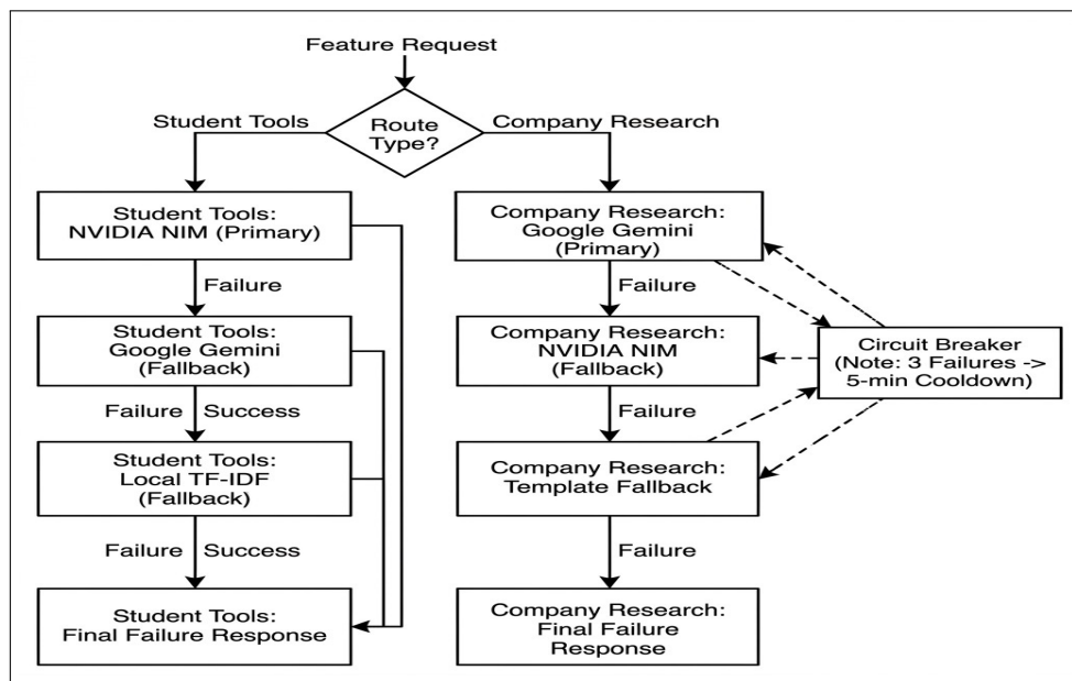
Figure 2. Multi-model orchestration and fallback chain
