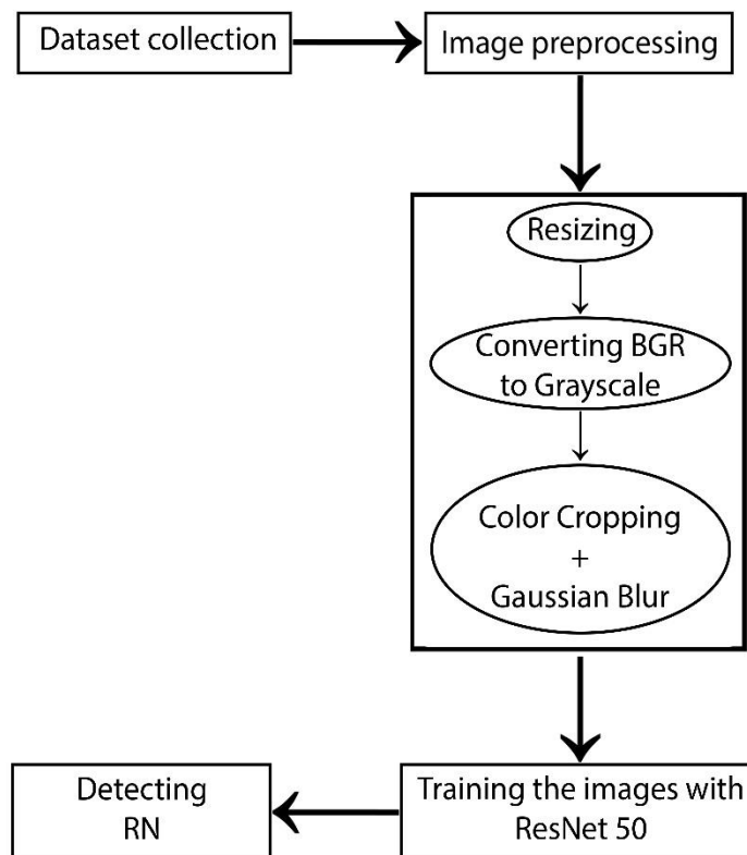
Figure 2. Architecture Diagram
