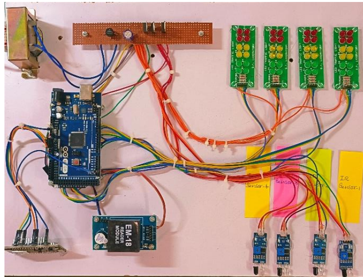
Figure 4.3. Hardware setup
