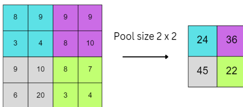
Figure 2. Overview of Global Average Pooling 2D
