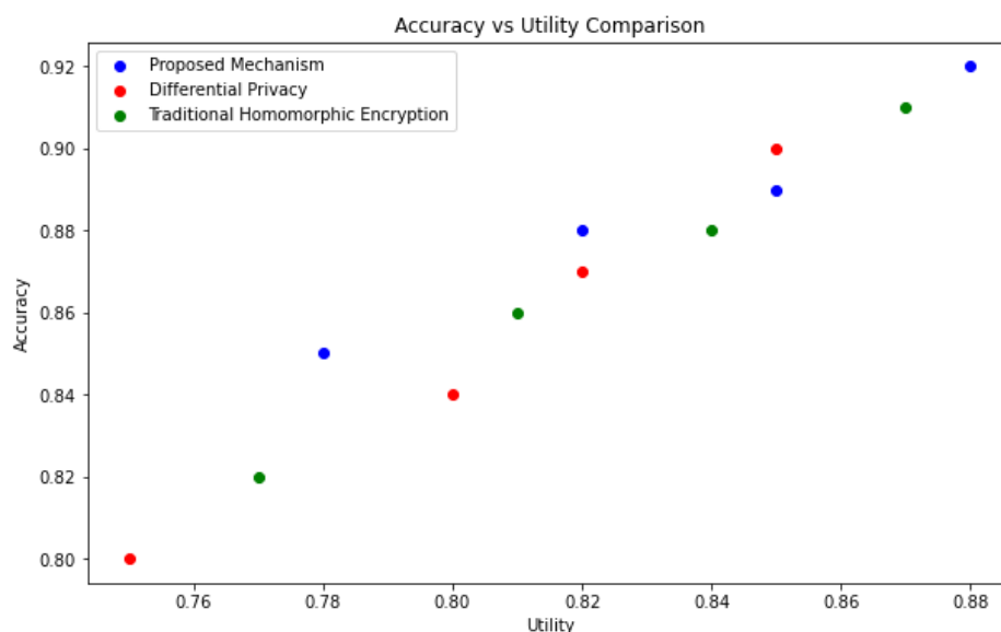
Figure 3. Accuracy versus Data Utility Comparison
