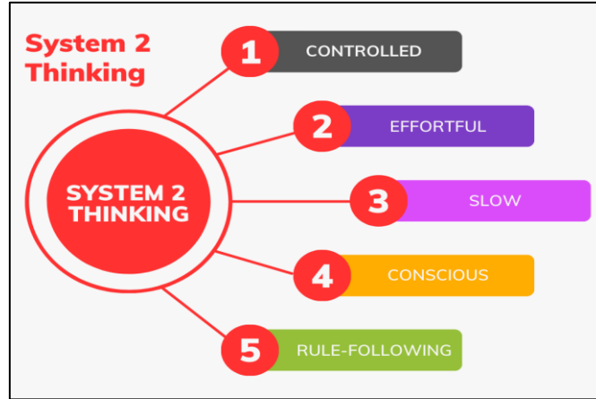
Figure 2. System 2 Thinking
