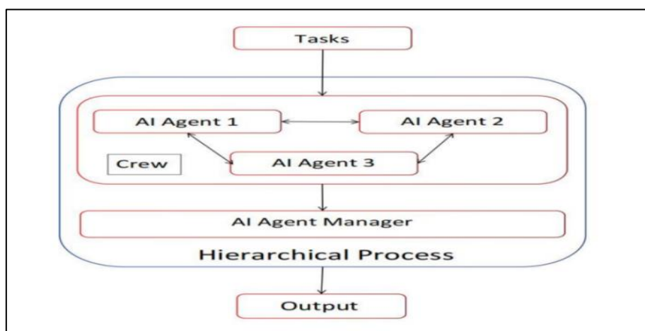
Figure 5. Hierarchical Process
