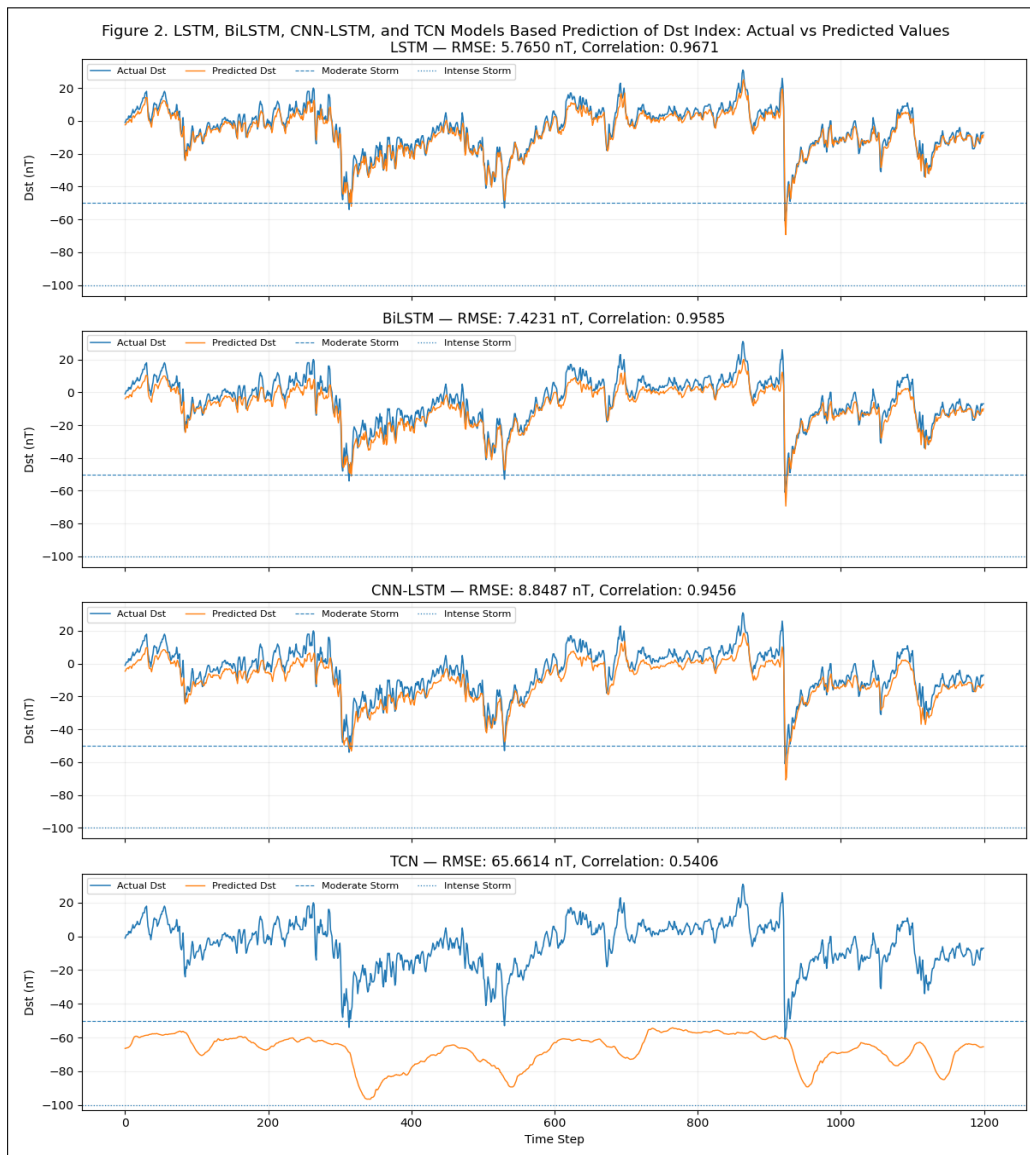
Figure 1. LSTM, BiLSTM, CNN-LSTM, and TCN models-based prediction of Dst index: actual versus predicted values
